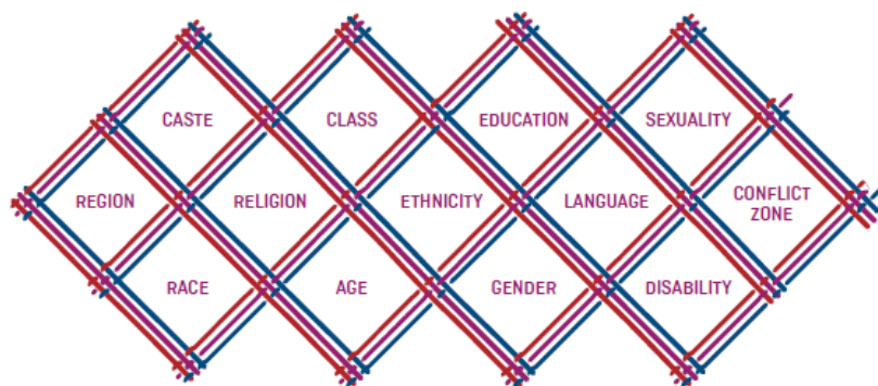
Diagram 3. Intersecting identities
